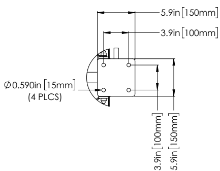
MOUNTING PLATE VIEW (MOUNTING HARDWARE NOT INCLUDED)
